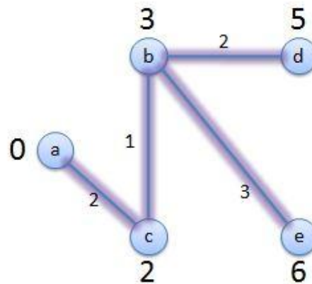
Figure 3.3: Final Shortest paths found using Dijkstra's Algorithm
