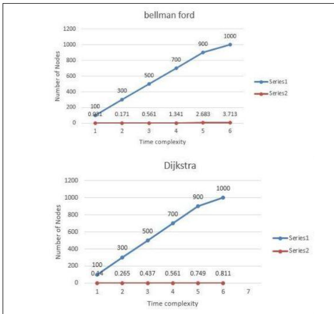
Figure 4.2: Time complexity comparison shown in graph between Bellman-Ford and Dijkstra's Algorithm
