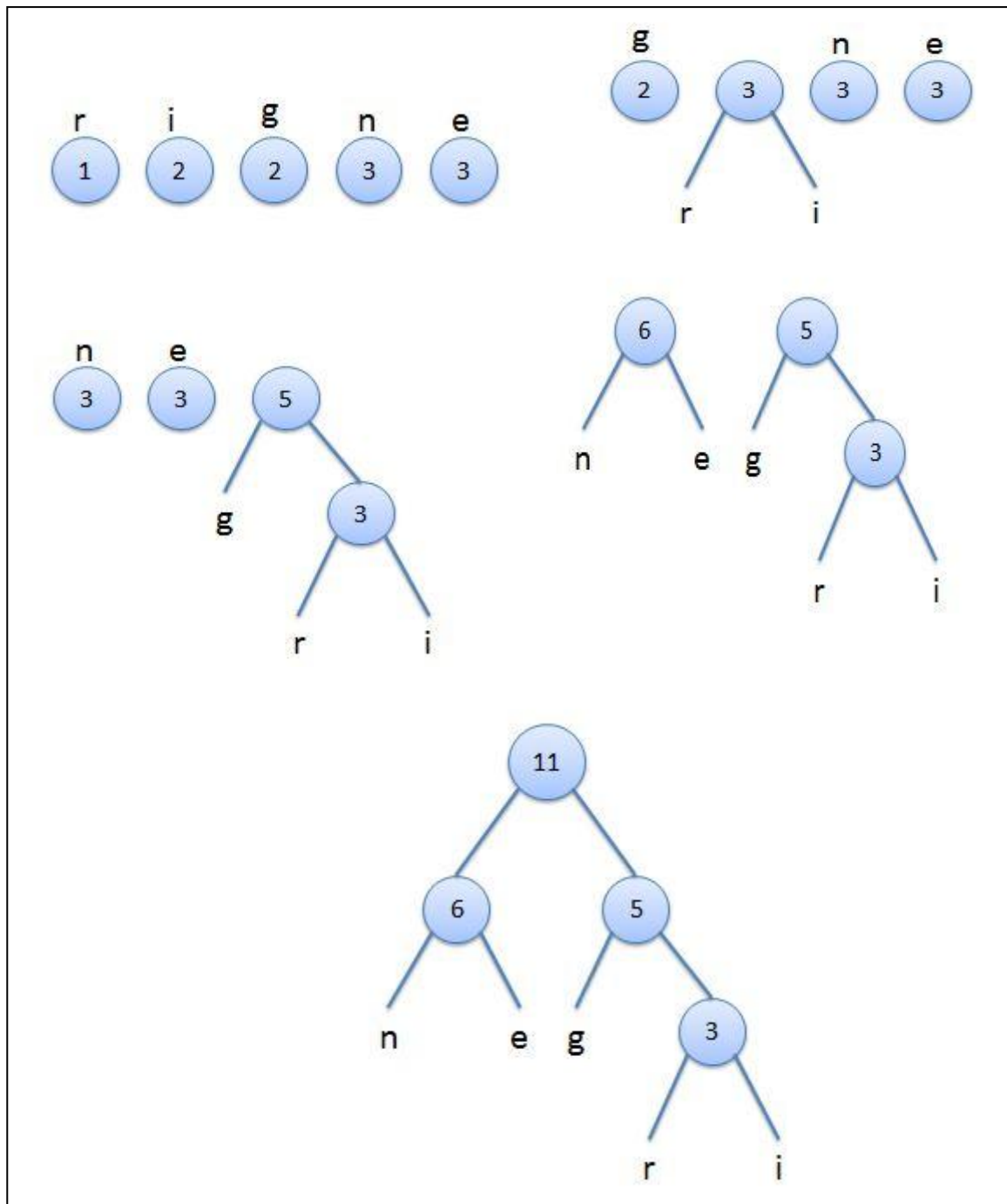
Figure 3.7: Huffman working process
