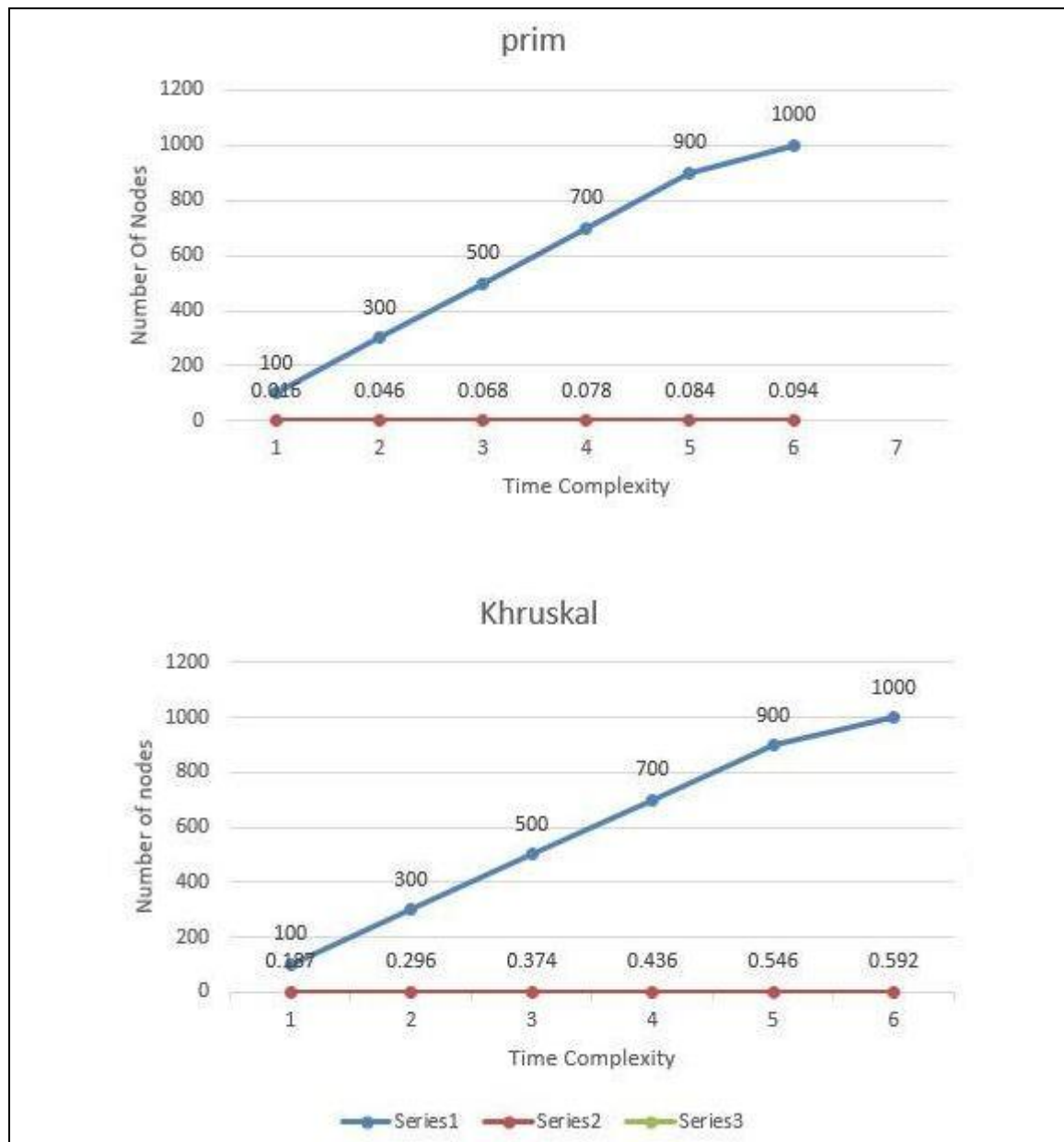
Figure 4.1: Time complexity comparison shown in graph between Prim's and Kruskal's Algorithm
