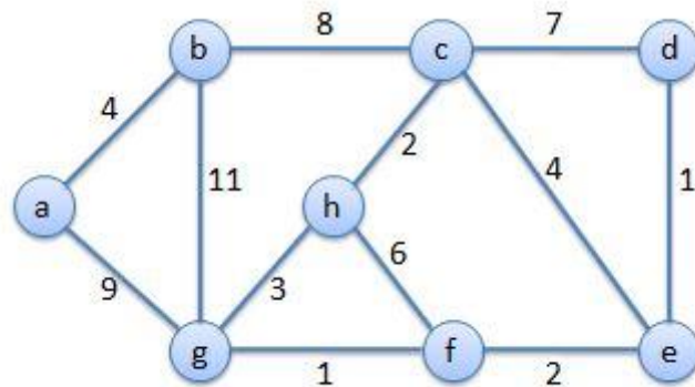
(a) The original graph
