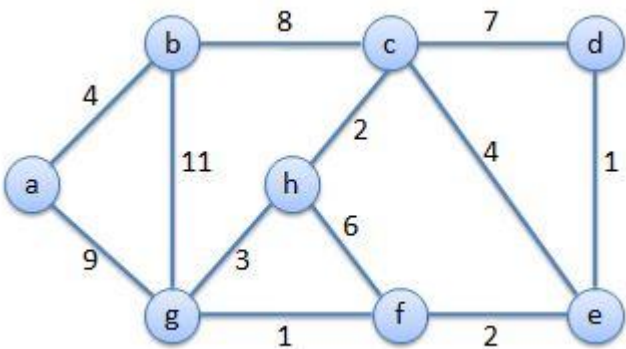
(a) The original graph
