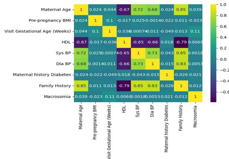
Figure 6 Graphical representation of the correlation coefficients between pairs of variables in a dataset.
