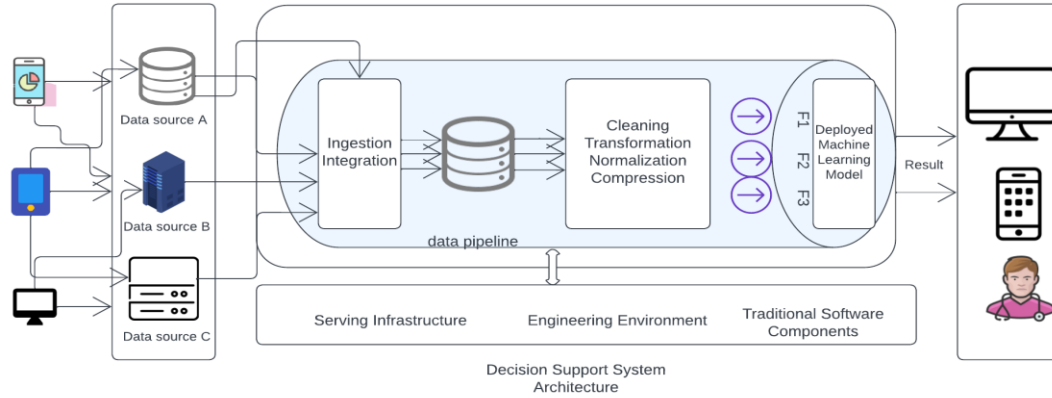
Figure 12 Deployed Machine learning model Architecture.
