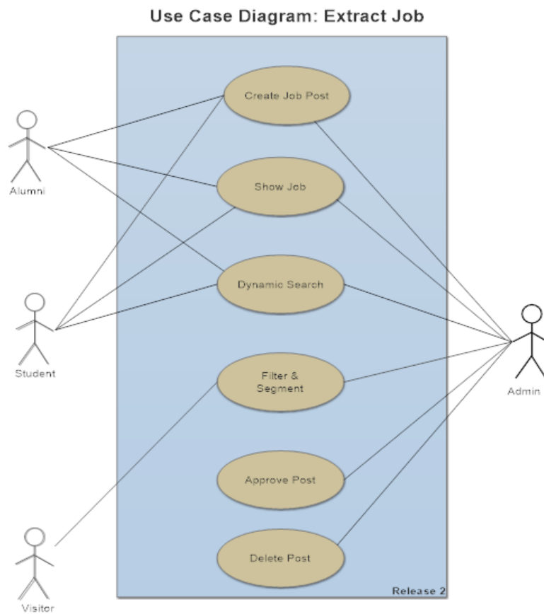
Figure 3.2: Use Case of Job Portal Module
