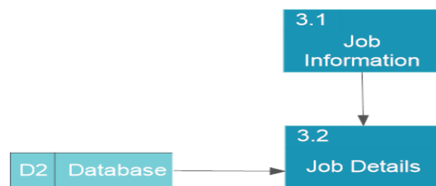
Figure 3.9: Level 3 DFD
