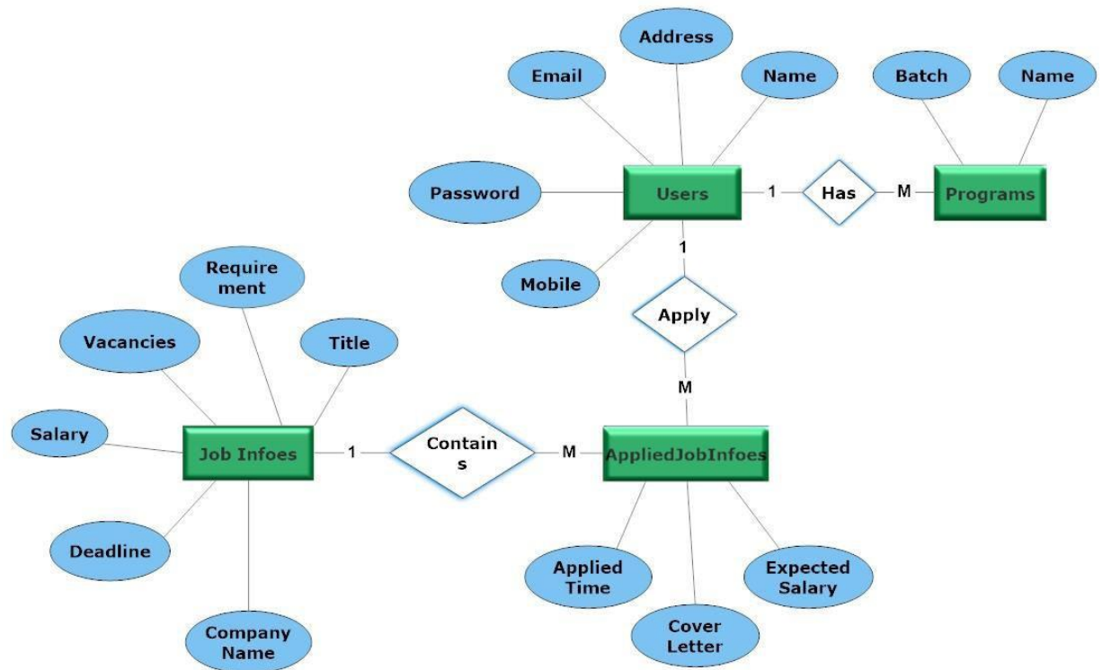
Figure 3.4: Entity Relationship Diagram (ERD)
