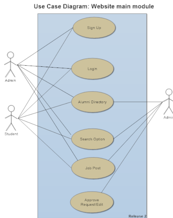
Figure 3.1: Use Case of Main Modules
