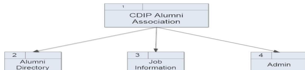
Figure 3.7: Level 1 DFD
