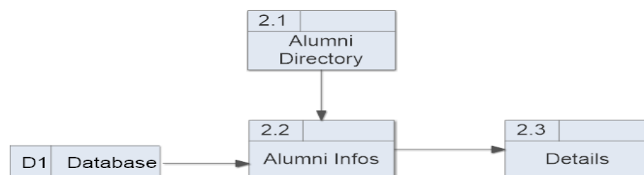
Figure 3.8: Level 2 DFD
