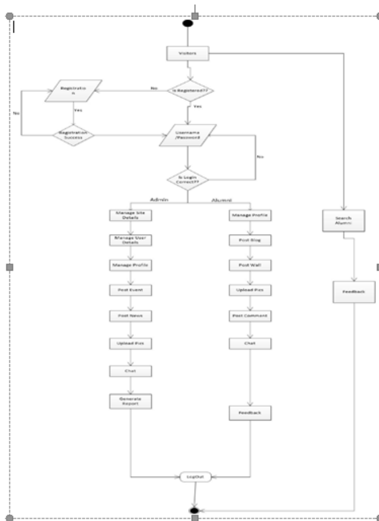
Figure 3.6: Activity Diagram
