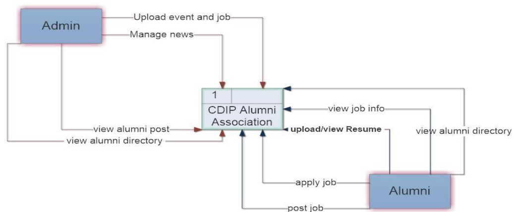
Figure 3.10: Context Diagram
